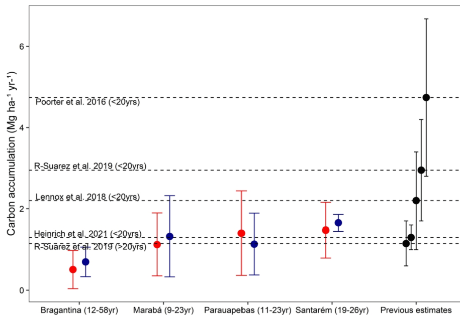
Fig. 4. Comparisons of contemporary (darkblue) and lifetime (red) carbon accumulation rates of secondary forests across regions and with others estimates (black) for the Eastern Amazon (Poorter et al., 2016; Lennox et al., 2018; Heinrich et al., 2021) and South America (Requena Suarez et al., 2019). Points represent the average rates ( \pm 95\% CI). (For interpretation of the references to colour in this figure legend, the reader is referred to the web version of this article.)
